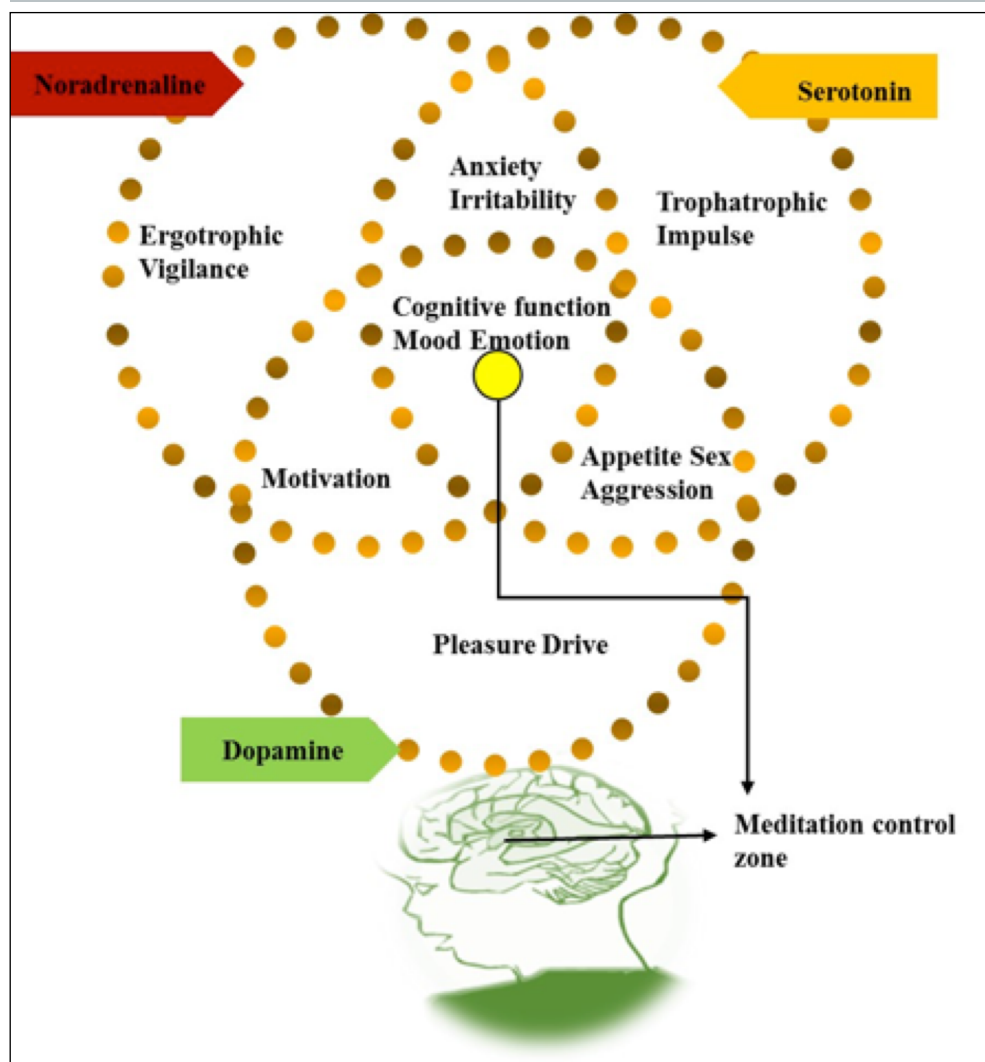
Figure 2: The illustration provides a general view of the different roles of the common neurotransmitters—Noradrenaline (Norepinephrine), Dopamine and Serotonin. It is vital that the neurotransmitters are in balance for optimum common cognitive and physiological functionalities, and this can be achieved when the brain is in a meditative state.
