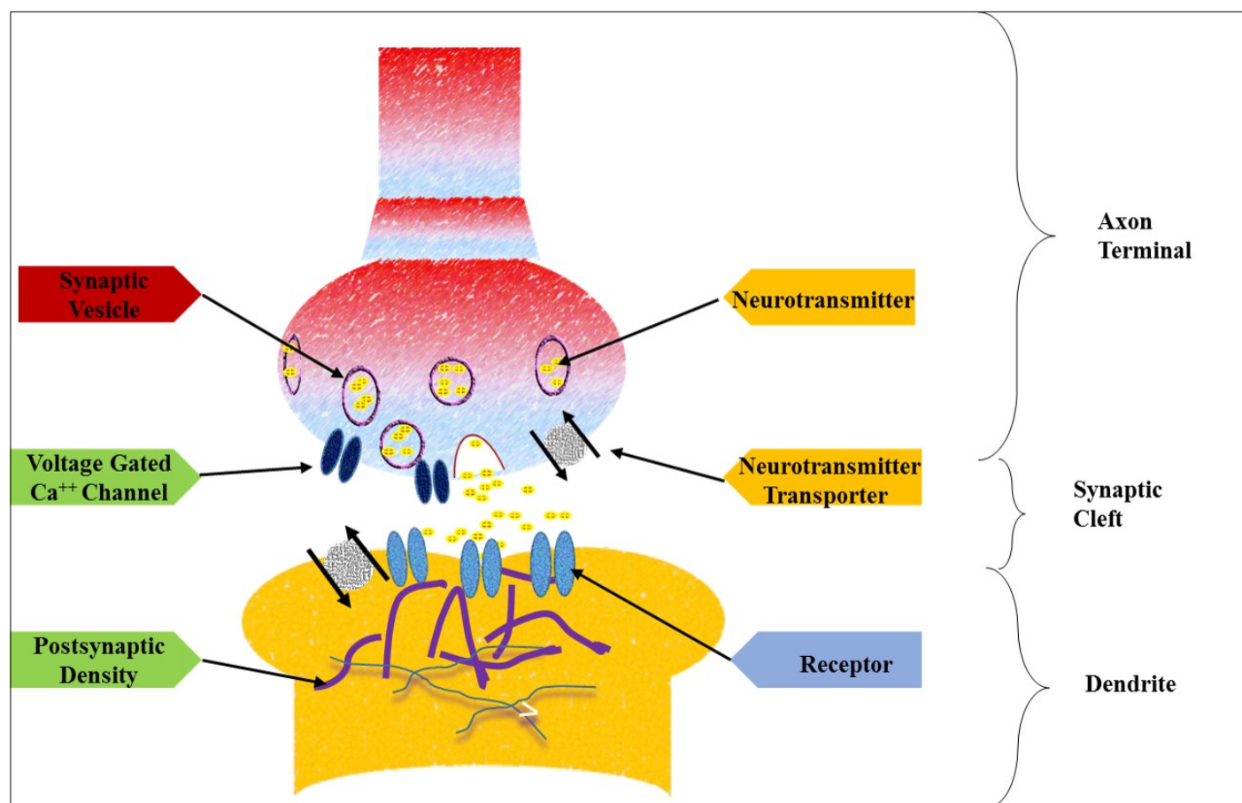
Figure 1: Illustration of a Chemical Synapse. Neurotransmitters are essential brain chemicals that help relay information between neurons. At the synaptic cleft, the neurotransmitters are released from the axon terminal of one neuron. The released neurotransmitters then bind to the receptor sites of the postsynaptic neuron.
