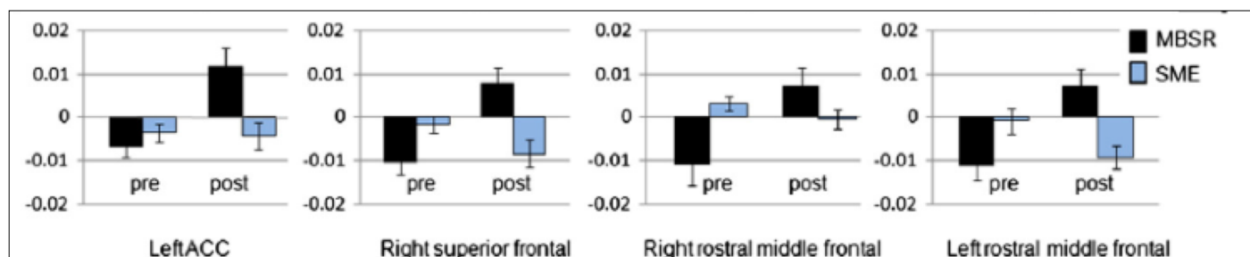
Figure 3: A pre- and post- comparison of the functional connectivity of GAD patients between the individuals who underwent a Mindfulness Based Stress Reduction Program (MSBR) and those who participated in Stress Management Education (SME) [35].
